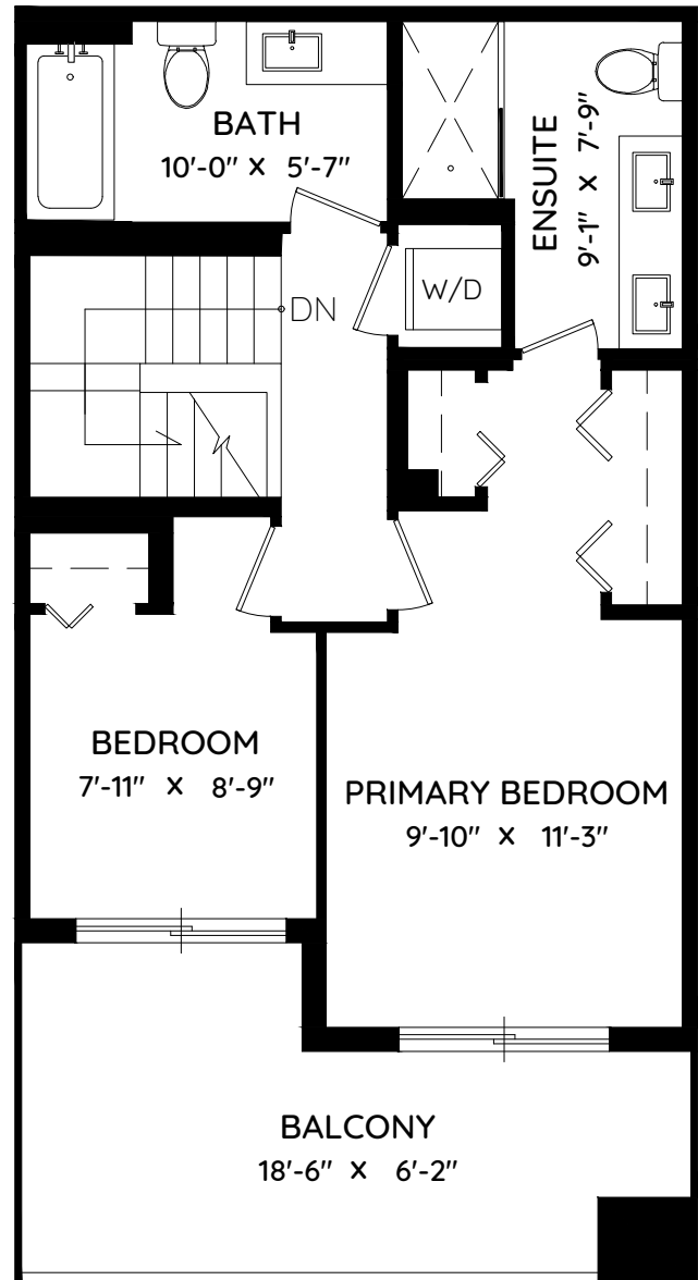
UPPER FLOOR 523 SQ.FT. CH: 7'-5"
