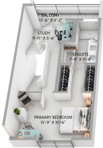
Level Four - 519 sq.ft. Ceiling height - 9' 0"
